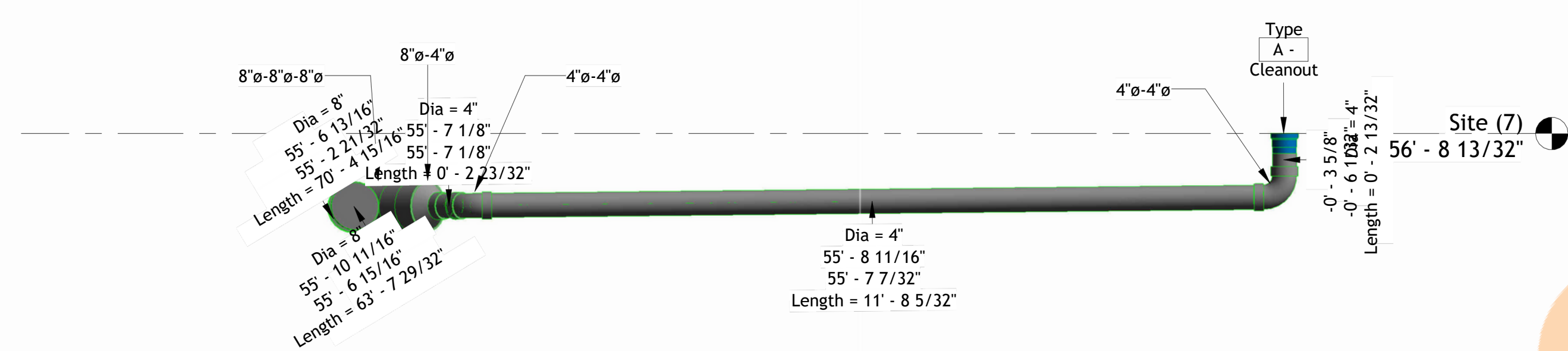
3 Elevation - Site 7 1/2" = 1'-0"
